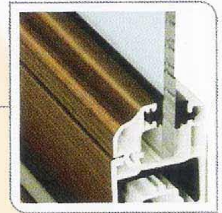
Aesthetic appearance with decorative Glazing Bead.
