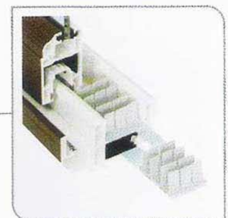
Preventing water leakage led by mal-screwing from adopting new clip-on system in bottom frame.
