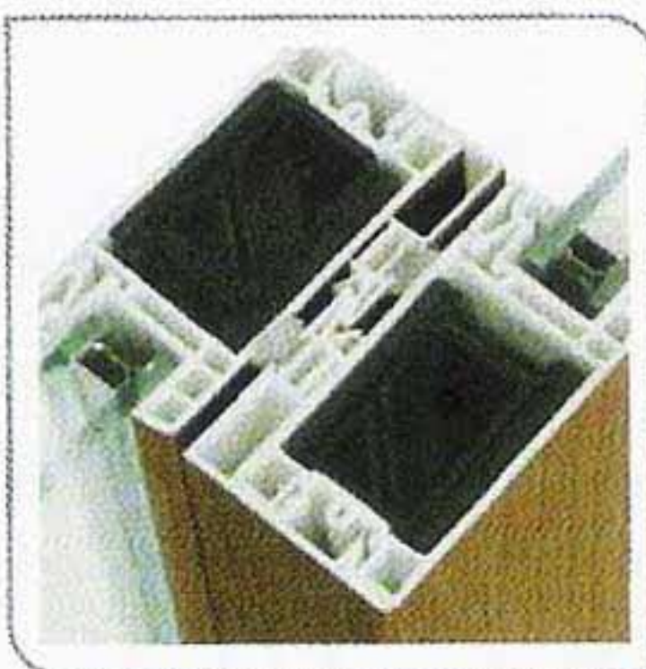
Structurally enhanced panel (option)
