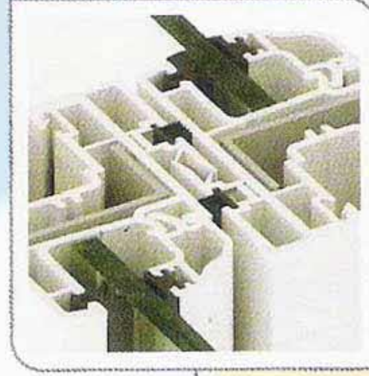
Minimizing an inflow of dust by double sealed interlocking parts.
