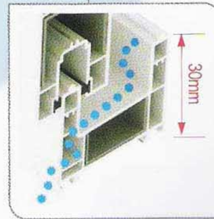
Enhanced water tightness with raised track rail system (30mm) & stair type structure.
